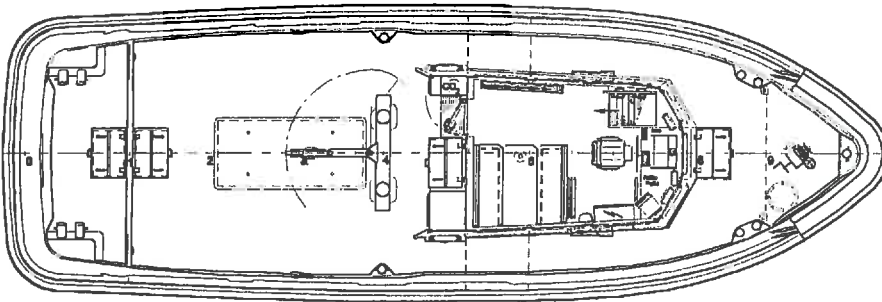
MAINDECK/ADALÞILFAR
